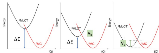
Fig. 9 Schematic representation of the ^3\text{MLCT} and the ^3\text{MC} states approximated as harmonic potentials along an effective structural coordinate Q . When the energy gap \Delta E decreases (left to right), the barrier V_b between ^3\text{MLCT} and ^3\text{MC} increases, leading to a longer ^3\text{MLCT} lifetime.
