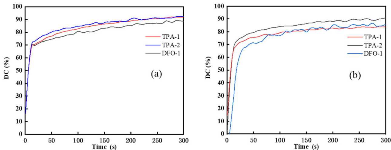
Fig. 3 Photopolymerization kinetics of the chalcones/lod/EDAB systems (chalcones: 0.1 wt%; lod: 1.0 wt%; EDAB: 1.0 wt%, TMPTA as monomer) under different light sources (a) 365 nm LED, (b) 405 nm LED.
