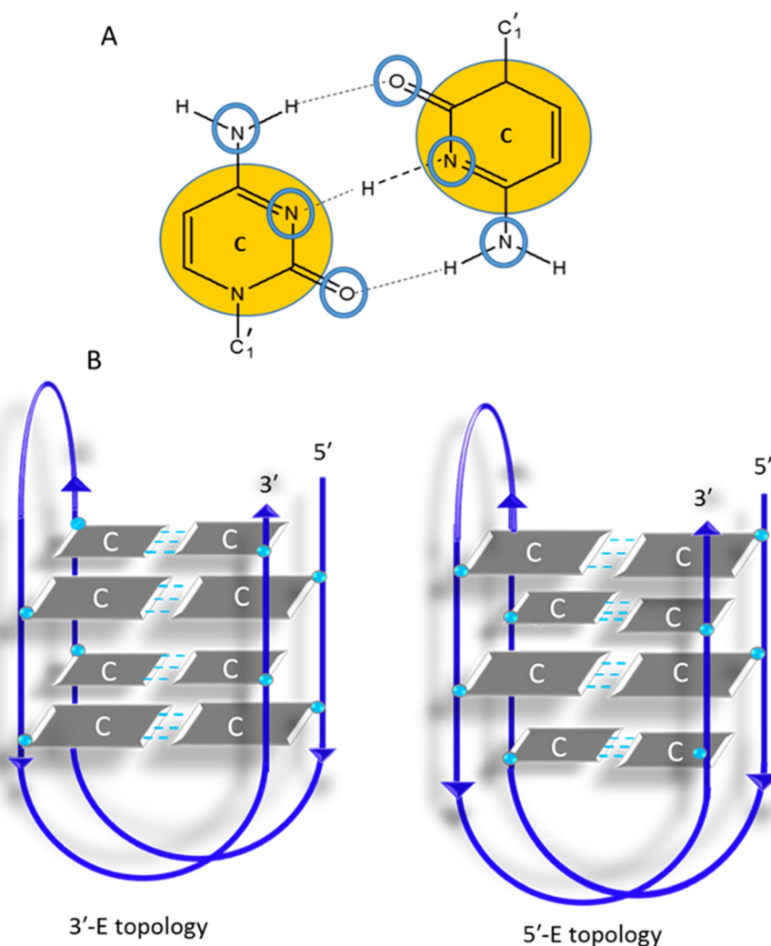
Fig. 1 The C : C + base pair structure and stacking between intercalating C : C + base pairs (A), and two intercalation topologies of an intermolecular i-motif DNA structure (B).
