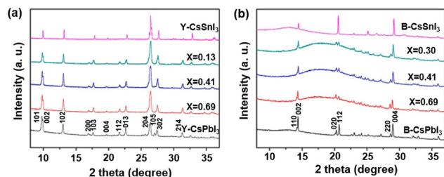
Fig. 7 XRD patterns of (a) Y-phase CsPb x Sn 1-x I 3 NWs and (b) B- \gamma phase CsPb x Sn 1-x I 3 NWs. Reproduced from ref. 78 with permission from the American Chemical Society. Copyright 2018.
