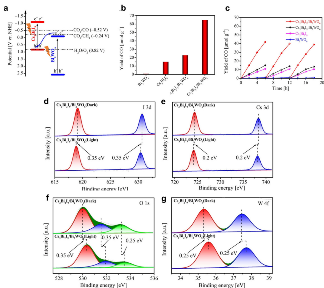
Fig. 8 (a) The band structures for \text{Cs}_3\text{Bi}_2\text{I}_9 and \text{Bi}_2\text{WO}_6 . (b) The yield of CO generated from photocatalytic \text{CO}_2 reduction after 9 h of irradiation. (c) Recycling stability tests of as-prepared samples with three cycles. (d–g) High-resolution XPS spectra of \text{Cs}_3\text{Bi}_2\text{I}_9/\text{Bi}_2\text{WO}_6 in the dark or under 300 W Xe lamp irradiation with a 400 nm filter: (d) I 3d, (e) Cs 3d, (f) O 1s, and (g) W 4f. Reproduced with permission from ref. 42. Copyright 2021 Wiley-VCH.
