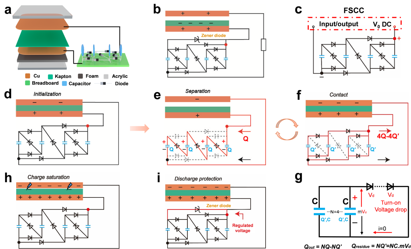
Fig. 1 Working principle of the fractal structured charge-excitation TENG. (a) Schematic illustration of the FSCC-TENG with an FSCC of 4 = 2 \times 2 structure. (b) Whole circuit system of the FSCC with a Zener diode for the FSCC-TENG. (c) Input/output node and scheme of the FSCC. (d) Charge distribution of FSCC-TENG at the initial state. (e–g) Charge-excitation process during periodic contact-separation cycles. (h and i) Schematic charge distribution in the FSCC-TENG at the (h) charge saturation, and (i) discharge protection using a regulator diode.
