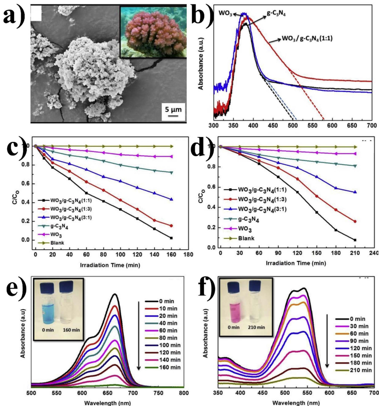
Fig. 12 (a) SEM image of \text{WO}_3/\text{g-C}_3\text{N}_4 (-1:1), (b) DRS of \text{WO}_3/\text{g-C}_3\text{N}_4 using various photocatalysts (c) \text{C}/\text{C}_0 MB and (d) \text{C}/\text{C}_0 RbX. (e) UV-Vis spectra at different time intervals under visible light for the degradation of MB and (f) RbX using \text{WO}_3/\text{g-C}_3\text{N}_4 (-1:1) (reproduced with permission from ref. 120 Copyright 2019, Elsevier).
