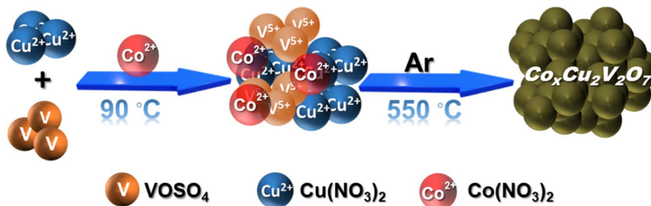
Scheme 1 Schematic illustration showing the formation method of Co 2+ doped Cu 2 V 2 O 7 .
