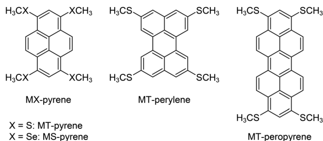
Fig. 1 Molecular structures of 1,3,6,8-tetrakis(methylthio)- and 1,3,6,8-tetrakis(methylseleno)-pyrene and (MT- and MS-pyrene), 2,5,8,11-tetrakis(methylthio)peryene (MT-peryene), and 1,3,8,10-tetrakis(methylthio)peropyrene (MT-peropyrene).
