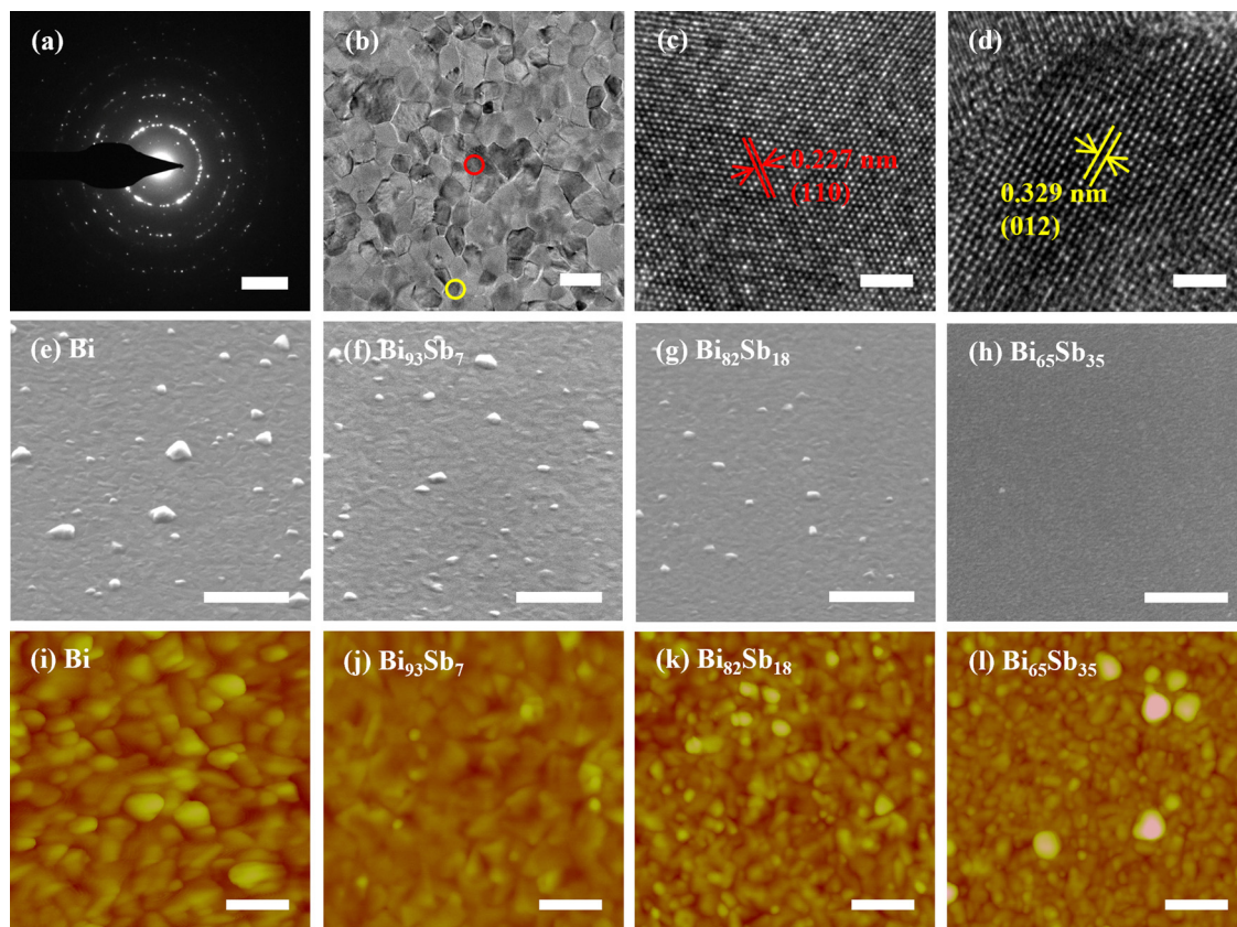
Fig. 3 Atomic structure and morphology of 2D bismuth antimonide. (a) SAED pattern and (b–d) TEM images of 17 nm Bi 82 Sb 18 ; the lattice fringes in (d) correspond to the red circle and the yellow circle in (b). (e–h) SEM and (i–l) AFM images of 2D bismuth antimonide. Color scale for the AFM images is –10 to 10 nm. Scale bar: (a) 5 nm –1 , (b) 50 nm, (c and d) 2 nm, (e–h) 500 nm, (i–l) 100 nm.
