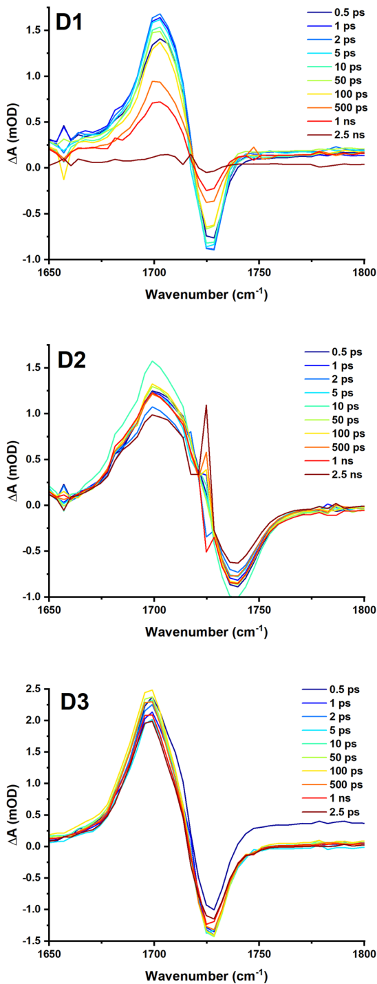
Fig. 8 TRIR spectra of D1, D2 and D3 in DCM following excitation at 525, 500 and 500 nm respectively (2 mW, OD@_{\lambda_{ex}} = \sim 0.6 ), collected with the pump set to magic angle ( 54.7^\circ ) with respect to the probe. The time delay between the pump and probe for each spectrum is shown in the legend. Kinetic traces are shown in the ESI.†
