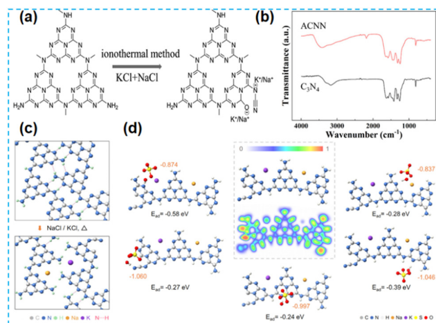
Fig. 5 (a) Schematic illustration of the procedure for introducing alkali metal dopants and N vacancies on CN. (b) FTIR spectra of ACNN (alkali metal dopants and N vacancies on CN) and C 3 N 4 . 37 (c) Proposed structure evolution of PCN during the thermal treatment process in alkali metal salts. (d) Color-filled map of calculated ELF of ACN (alkali metal salts modified carbon nitride). 38
