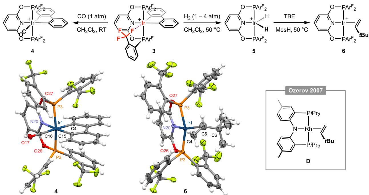
Fig. 3 Reactivity of complex 3; MesH = mesitylene and [BAR 4 ] − counter ions omitted for clarity. Solid-state structures of 4 and 6 drawn with thermal ellipsoids at 30% probability and without solvent molecules. Selected metal-based bond lengths (Å) and angles (°): 4, Ir1–P2, 2.3300(7); Ir1–P3, 2.3243(7); Ir1–N20, 2.102(2); Ir1–C4, 2.092(3); Ir1–C15, 2.072(3); Ir1–C16, 1.958(3); C16–O17, 1.123(4); P2–Ir1–P3, 159.85(2); N20–Ir1–C15, 171.25(10); C4–Ir1–C16, 177.09(11); 6, Ir1–P2, 2.2657(11); Ir1–P3, 2.2704(12); Ir1–N20, 2.058(4); Ir1–Cnt(C4,C5), 2.110(12); C4–C5, 1.304(12); P2–Ir1–P3, 156.46(5); N20–Ir1–Cnt(C4,C5), 175.3(4); C4–C5–C6, 130.6(10); D, Rh–Cnt(C=C), 2.051(3); C=C, 1.360(10); N–Rh–Cnt(C=C), 174.27(14); C=C–C, 127.7(5). 15 Cnt = centroid.
