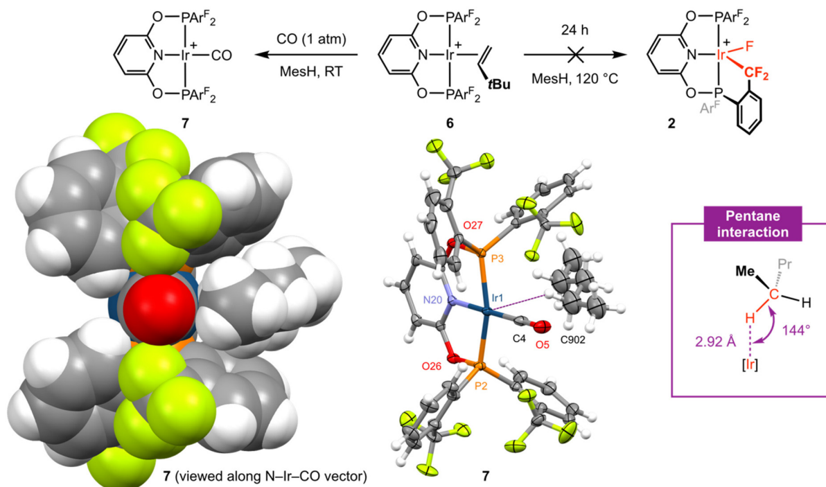
Fig. 4 Reactivity of complex 6; MesH = mesitylene and [BAR 4 ] − counter ions omitted for clarity. Solid-state structures of 7 drawn in space fill (left) and with thermal ellipsoids at 30% probability (middle); CH 2 Cl 2 solvent molecule not shown. Selected metal-based bond lengths (Å) and angles (°): 7, Ir1–P2, 2.2720(7); Ir1–P3, 2.2828(7); Ir1–N20, 2.050(2); Ir1–C4, 1.858(3); C4–O5, 1.137(4); P2–Ir1–P3, 161.38(3); N20–Ir1–C4, 177.01(13); Ir1...C902, 3.759(11).
