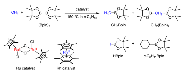
Scheme 6 Catalytic borylation of \text{CH}_4 by a Ru or Rh complex in \text{c-C}_6\text{H}_{12} at 423 K. 25
