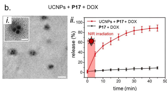
Fig. 25 Light-responsive micelles containing DASAs. (a) Schematic illustration of micellization process from amphiphilic polymeric compounds and structures of DASA-modified polymers used for micelle formation. (b) Micelles of P17 assembled with upconversion nanoparticles (UCNPs) that are responsive to NIR light. (i) Transmission electron microscopy (TEM) image of micelles loaded with an average of 2-4 UCNPs with the scale bar of 150 nm (inset: 75 nm). (ii) Release of doxorubicin (DOX) from micelles with and without UCNPs after 5 min NIR irradiation (808 nm laser, 2 W cm -2 ). Release was quantified by monitoring the fluorescence of DOX in the supernatants over time. Figures adapted with permission from ref. 134 Copyright 2021 Elsevier. (c) Ellipticine release from micelles made from P18 in water at 37 °C. UV-Vis absorption of DASA-modified micelles (518 nm, black trace) and ellipticine drug release (red trace) for 3 irradiation cycles with a 530 nm LED (2.15 W intensity; 2 h ON, 2 h OFF). The release from the micelles was quantified by monitoring the polarity-sensitive fluorescence of ellipticine in situ . Figure adapted with permission from ref. 133 Copyright 2019 Royal Society of Chemistry. (d) Nile red release from micelles of P19 assembled with UCNPs that are responsive to NIR light. The release was monitored via a dialysis method and the graph displays the increase in Nile red fluorescence intensity (at 640 nm, λ ex = 550 nm) in the receiver compartment over time for micelles under light exposure (0.2 W 808 nm laser, 6.37 W cm -2 , or 532 nm LED, 12.8 mW cm -2 ) and in the dark. The inset shows a TEM image of a micelle after NIR irradiation (three UCNPs covered by the polymer layer). Figures adapted with permission from ref. 132 Copyright 2021 John Wiley and Sons.
