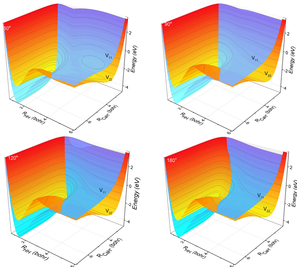
Fig. 1 3D PESs of the non-adiabatic states V_{\text{d}}^{11} and V_{\text{d}}^{22} for Ca-H-H with bond angles of 60.0°, 90.0°, 120.0° and 180.0°.
