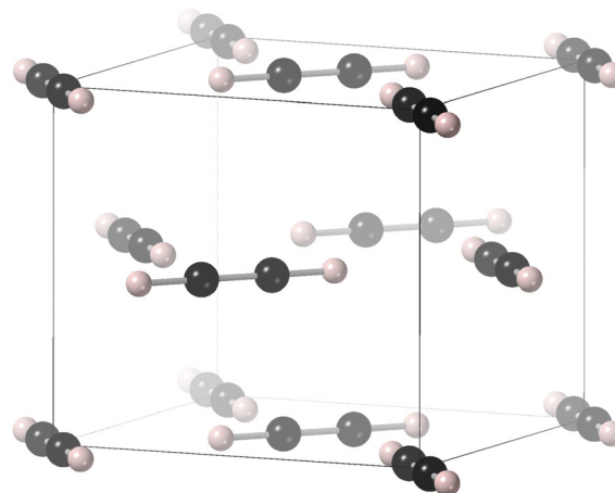
(a) Orthorhombic phase
