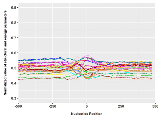
Fig. 7 Normalised and combined structure and energy graph for all sequences (5561) containing TSS from Caenorhabditis elegans .
