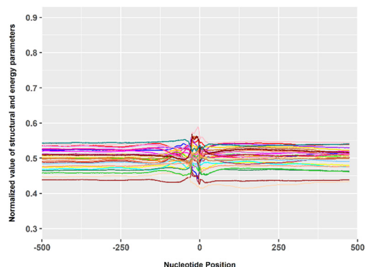
Fig. 6 Normalised and combined structure and energy graph for all sequences (197 356) containing TSS from the 8 eukaryotic species.
