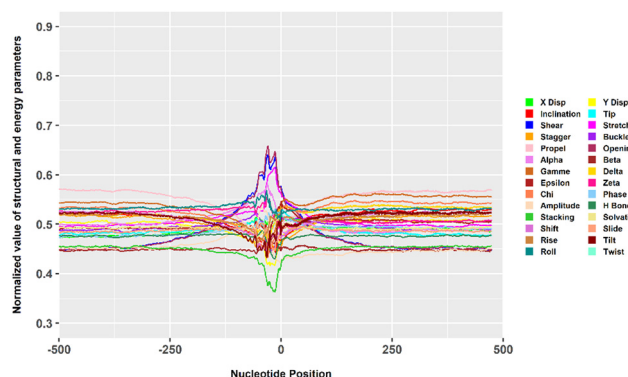
Fig. 3 Normalised and combined structure and energy graph for all sequences (16 519) containing TSS from 12 prokaryotic organisms.
