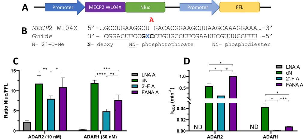
Fig. 10 Effect of -1 nucleoside analogs on cellular editing as measured by dual luciferase assay compared to effect on in vitro editing. (A) Schematic representation of dual luciferase plasmid with target site MECP2 W104X upstream of reporter luciferase Nluc. FFL expressed independently of editing. (B) Modification pattern for guide oligonucleotides used in cellular editing. (C) Relative Nluc/FFL luminescence signals observed for guide oligonucleotides with varying -1 nucleoside analogs and either 10 nM of guide and overexpressed ADAR2 or 30 nM of guide and overexpressed ADAR1 in HEK293T cells. (D) Comparison of in vitro deaminations of four -1 nucleoside analogs used for cell studies. gRNAs follow modification pattern found in Fig. 3. Information on in vitro deamination conditions and analysis can be found in Fig. 4 (ADAR2) or Fig. 5 (ADAR1). Error bars, s.d. ( n \geq 5 biological replicates). A Grubbs test for outliers was conducted at p = 0.05 significance level. A two-tailed Welch's t test was conducted, where * p < 0.05 , ** p < 0.01 , *** p < 0.001 , **** p < 0.0001 .
