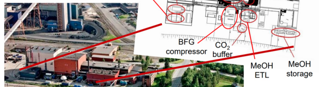
Fig. 21 Layout of the FReSMe project. 89
