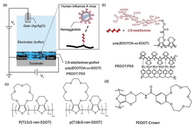
Fig. 6 (a) Schematic of the OECT device, employing the poly(EDOTOA-co-EDOT)/PEDOT:PSS composite as the active channel material. (b) Chemical structure of the 2,6-sialyllactose functionalized EDOT derivative. Reproduced from ref. 72 with permission from Elsevier. (c) Chemical structures of crown ether functionalized PEDOT copolymer. 73 (d) Chemical structure of PEDOT-Crown. 74
