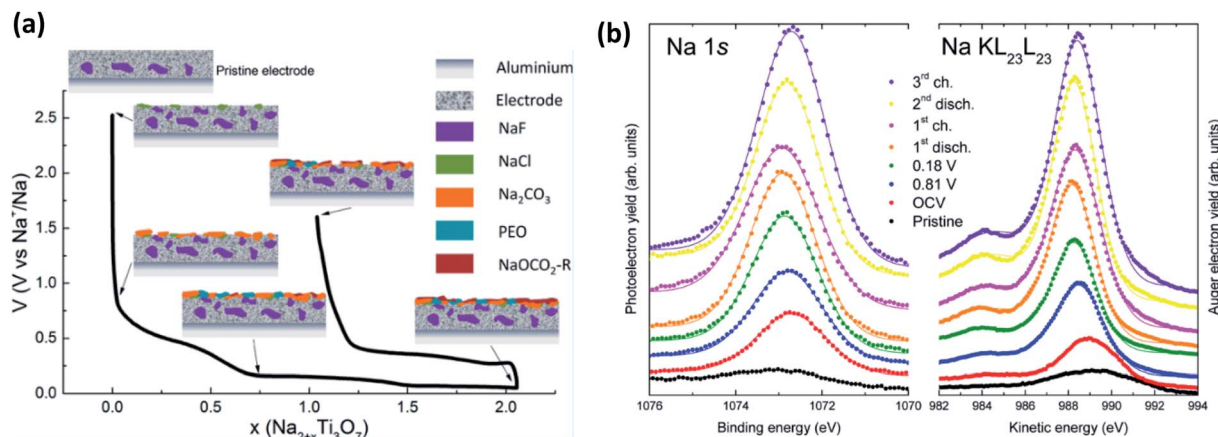
Fig. 13 (a) The composition and evolution of the SEI on Na 2 Ti 3 O 7 electrodes as determined by XPS. (b) Na 1s XPS spectra and Na KL 23 L 23 Auger transition spectra for electrodes at different states of charge. Reprinted with permission from ref. 143. Copyright 2015 American Chemical Society.
