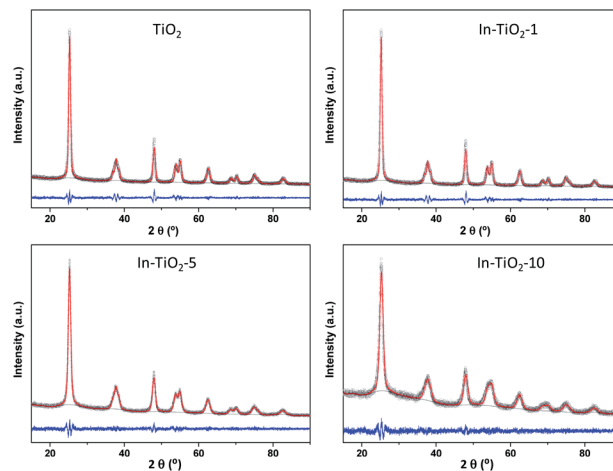
Fig. 1 Pawley refinement of X-ray diffractograms of In-doped and bare TiO 2 samples. Circles: experimental data; red line: fitting; grey line: background; blue line: exponential-simulation subtraction.
