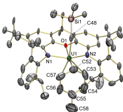
Fig. 4 X-ray crystal structure of [(\text{XA}_2)\text{U}(\text{CH}_2\text{SiMe}_3)(\eta^6\text{-C}_6\text{H}_5\text{Me})][\text{B}(\text{C}_6\text{F}_5)_4]\cdot\text{toluene} ( 3-toluene ), with thermal ellipsoids at 50% probability. Hydrogen atoms, the borate anion and a non-coordinated toluene solvent molecule are omitted for clarity. Selected bond distances (Å) and angles (°): U(1)–O(1) 2.417(9), U(1)–N(1) 2.22(1), U(1)–N(2) 2.21(1), U(1)–C(48) 2.36(2), U(1)–C(52) 3.05(2), U(1)–C(53) 3.13(2), U(1)–C(54) 3.47(2), U(1)–C(55) 3.78(2), U(1)–C(56) 3.70(2), U(1)–C(57) 3.36(2), U(1)–C arene ave. 3.42, U(1)–Centroid 3.14, C(55)–C(58) 1.46(3), U(1)–C(48)–Si(1) 136.8(7), O(1)–U(1)–C(48) 88.8(4), N(1)–U(1)–N(2) 128.0(4).
