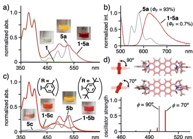
Fig. 5 (a) UV-visible spectra and photographs (5 : 1 water/AN, r.t.) of 1·5a, 1, and 5a (in \text{CH}_2\text{Cl}_2 ) and (b) their fluorescence spectra ( \lambda_{\text{ex}} = 500 nm) except for 1. (c) UV-visible spectra (5 : 1 water/AN, r.t.) of 1·5b, 1·5c, 5b (in \text{CH}_2\text{Cl}_2 ) and 5c (in DMSO). (d) Optimized structures of 5a with \phi = 90^\circ and 70^\circ and their predicted, electronic absorption bands. 15
