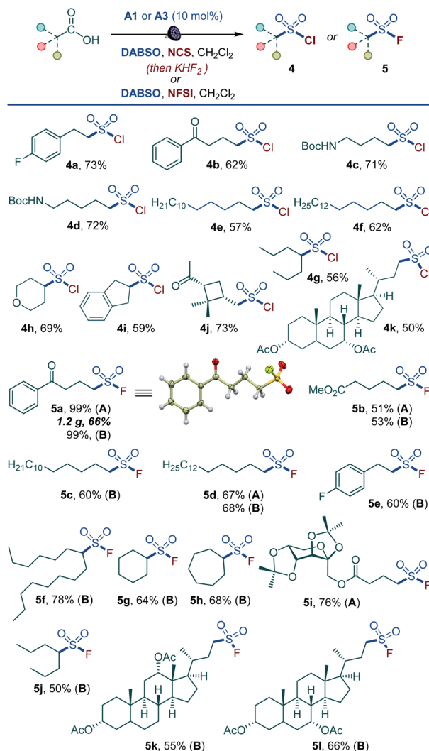
Scheme 3 Scope of the direct decarboxylative chloro- and fluoro-sulfonylation. Reaction conditions: carboxylic acid (0.3 mmol), \text{DABSO} (0.3–0.36 mmol), \text{A1} (10 mol%), N -chlorosuccinimide (NCS) (0.6–0.75 mmol), \text{CH}_2\text{Cl}_2 (6 mL), LED light (400 nm), 8–12 h, then purification for 4 , or (method A) 2 M \text{KHF}_2 (0.35 mL, 0.69 mmol), \text{MeCN} (2 mL), 50 °C, 3 h or 80 °C, 5 min. Method B: carboxylic acid (0.3 mmol), \text{DABSO} (0.45 mmol), \text{A2} (10 mol%), N -fluorobenzenesulfonimide (NFSI) (0.45 mmol), \text{CH}_2\text{Cl}_2 (6 mL), LED light (400 nm), 12 h.
