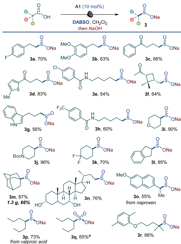
Scheme 2 Direct decarboxylative synthesis of alkyl sulfonates. Reaction conditions: carboxylic acid (0.3 mmol), \text{DABSO} (0.33 mmol), \text{A1} (10 mol%), \text{CH}_2\text{Cl}_2 (6 mL), LED light (400 nm), 12 h, then 1 M \text{NaOH} in \text{MeOH} (1 mL, 1.0 mmol), r.t., 10 min. a \text{Na}_2\text{S}_2\text{O}_8 (0.45 mmol) was added after treatment with \text{NaOH} .
