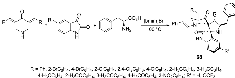
Scheme 30 Dispiropyrrrolidines 68 of antifungal properties.
