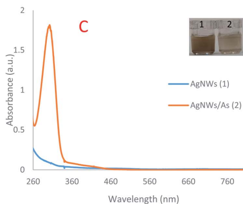
Fig. 1 The UV-Vis spectra of sensing probes in the presence and absence of arsenic (A) AgNPrs, Cys-capped AgNPrs, Met-capped AgNPrs; (B) AgNPrs, Cys-capped AgNPrs, Met-capped AgNPrs after 1 h; (C) AgNWs and (D) AgNWs after 1 h.
