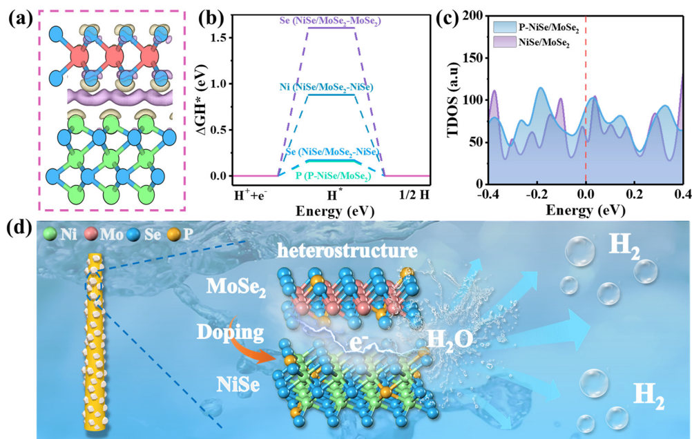
Fig. 6 (a) Charge density difference at the interface of the NiSe/MoSe 2 heterostructure. (b) Gibbs free-energy diagrams of NiSe/MoSe 2 and P-NiSe/MoSe 2 for \text{H} adsorption ( \text{H}^* ). (c) The calculated total electronic density of states (TDOS) of NiSe/MoSe 2 and P-NiSe/MoSe 2 . The Fermi level is set at 0 \text{ eV} as a reference. (d) Hydrogen production from the P-NiSe/MoSe 2 @NF catalyst promoted by the comprehensive strategy of preparing a heterostructure and P doping.
