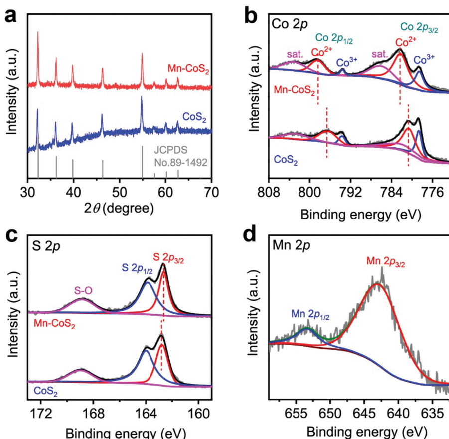
Fig. 3 Structural characterization of the as-prepared \text{CoS}_2 and \text{Mn-CoS}_2 : (a) XRD patterns; high-resolution XPS (b) Co 2p, (c) S 2p, and (d) Mn 2p spectra.
