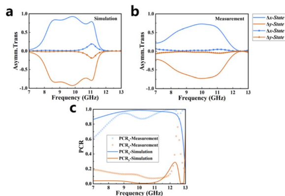
Fig. 6 Simulated (a) and measured (b) asymmetric transmission spectra and the (c) polarization conversion ratio for the chiral metasurface operating in different states.
