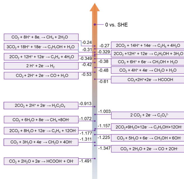
Fig. 7 \text{CO}_2\text{RR} at different standard potentials in aqueous solution at pH = 7.0, 1.0 atm, and 25°C. Reprinted with permission from ref. 26, copyright© 2019 The Royal Society of Chemistry.
