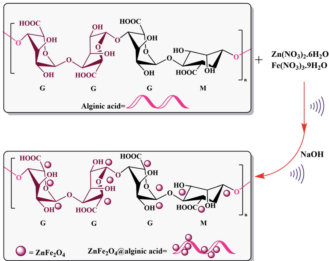
Fig. 8 Synthesis of \text{ZnFe}_2\text{O}_4@\text{alginate} . This figure was adapted with permission from Polyhedron , 2019, 171 , 193–202. 75
