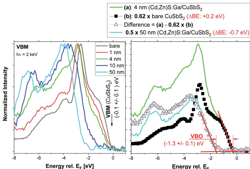
Fig. 7 Left panel: normalized HAXPES detail spectra (recorded with 2 keV) of the valence band maximum (VBM) region of the bare \text{CuSbS}_2 absorber and of the (\text{Cd,Zn})\text{S}:\text{Ga}/\text{CuSbS}_2 samples with buffer thicknesses varying from 1 nm to 50 nm. The VBM of the bare absorber (derived by linear extrapolation of the leading edge) is indicated. Right panel: visualization of subtracting the (properly scaled and shifted) spectrum of the bare \text{CuSbS}_2 absorber (b) from the 4 nm (\text{Cd,Zn})\text{S}:\text{Ga}/\text{CuSbS}_2 spectrum (a), resulting in a difference spectrum, representing the buffer related contribution to the VB spectrum. For comparison the (properly scaled and shifted) spectrum of the 50 nm (\text{Cd,Zn})\text{S}:\text{Ga}/\text{CuSbS}_2 sample is shown. The linear extrapolation of the leading edges of the (scaled and shifted) spectrum of the bare absorber and of the difference spectrum to derive the VBO is also depicted.
