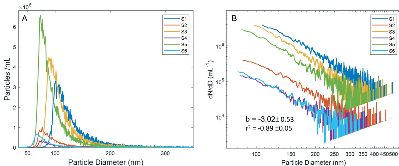
Fig. 2 A) Particle size distributions for ^{27}\text{Al} obtained by spICP-QMS. B) Reprocessed PSD data, with data normalized to number per nm ( dN/dD ) versus diameter and plotted in log space. The slope ( b ) and r^2 are an average of all samples; \pm 1 SD.
