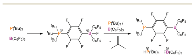
Scheme 2 Possible side-reaction between P(tBu)_3 and B(C_6F_5)_3 .
