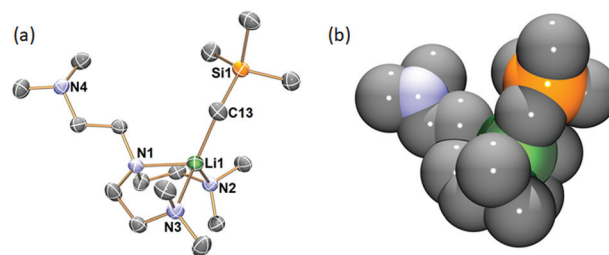
Fig. 1 (a) X-ray crystal structure of [\text{Li}(\text{CH}_2\text{SiMe}_3)(\kappa^3\text{-}N,N',N''\text{-Me}^6\text{Tren})] ( 1 ) at -123^\circ\text{C} with 50% probability ellipsoids. Hydrogen atoms are omitted and only the disordered component with the highest occupancy is shown for clarity. (b) Space filling presentation of 1 (grey: carbon; green: lithium; blue: nitrogen; coral: silicon). The selected bond distances (Å) and angles ( ^\circ ) are: Li1–C13 2.122(5) ; Li1–N1 2.177(4) ; Li1–N2 2.167(4) ; Si1–C13 2.189(4) ; Si1–C13–Li1 129.77(17) ; C13–Li1–N1 121.3(2) ; C13–Li1–N2 127.4(2) ; C13–Li1–N3 112.91(19) ; N2–Li1–N3 114.29(19) .
