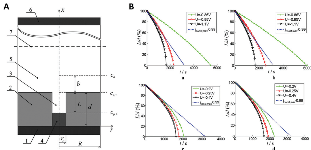
Fig. 9 (A) The model used for the simulation shows the metal deposition into a nanopore. Here, r_p is the radius of the nanopore, R the radius of the axisymmetric region of the simulation, d the thickness of the membrane, L the length of the empty pore, \delta the thickness of the outer diffusion layer, c_{p,+} the concentration of metal at the pore bottom, c_{s,+} the concentration of metal at the pore mouth c_0 the concentration of metal in the bulk solution, (1) is the metal contact, (2) the oxide template, (3) the empty pore, (4) the deposited metal, (5) the electrolyte, (6) the counter electrode and (7) the plane of the reference electrode. (B) Plots of the simulated unfilled pore length ( L ) versus the time under various potentials ( U ). Reproduced with permission from D. A. Bograchev, V. M. Volgin and A. D. Davydov, Electrochim. Acta , 2016, 207 , 247. 66
