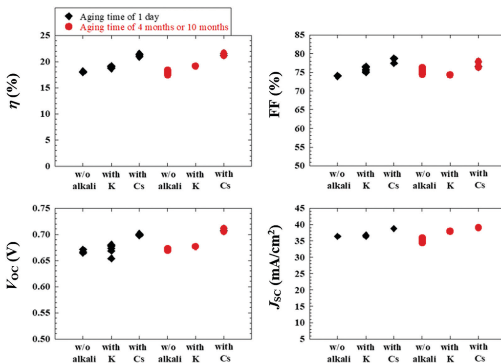
Fig. 17 Photovoltaic performance of the CdS-buffered CIGSSe solar cells using aged CIGSSe absorbers for aging times of 1 day, as well as 4 months or 10 months, where the absorbers were processed with and without the alkali (Cs or K) treatment.
