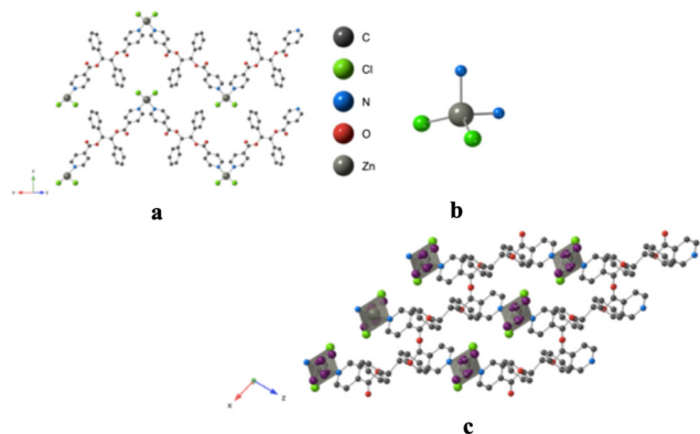
Fig. 4 For L-ZnCl 2 , portions of the X-ray structure showing a) the formation of the 1D zig-zag type coordination polymer, b) environment around the Zn 2+ cations and c) packing of consecutive networks in the xOz plane. Disordered chloroform solvent molecules are represented in purple. H atoms are not represented for clarity.
