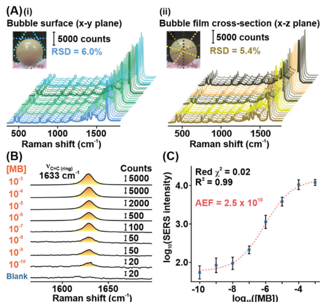
Fig. 3 (A) SERS spectra showing high signal homogeneity across different laser irradiation angles along the (i) bubble surface and (ii) bubble film cross-section. (B) SERS spectra showing the 1633 cm -1 peak changes with varying concentrations of MB. (C) Computing the detection limit and analytical enhancement factor of the Plasmonic bubble using the 1633 cm -1 peak.
