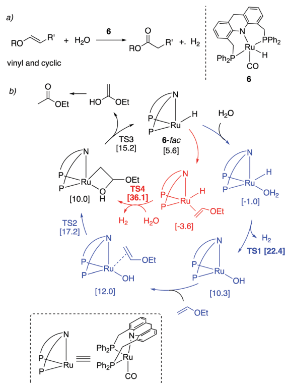
Fig. 23 (a) Enol ether to ester conversion catalyzed by complex 6 . (b) Reaction mechanism with stepwise inner-sphere and direct outer-sphere pathways. Calculated free energies (in brackets) are in \text{kcal mol}^{-1} with respect to 6-mer + ethyl vinyl ether + water.
