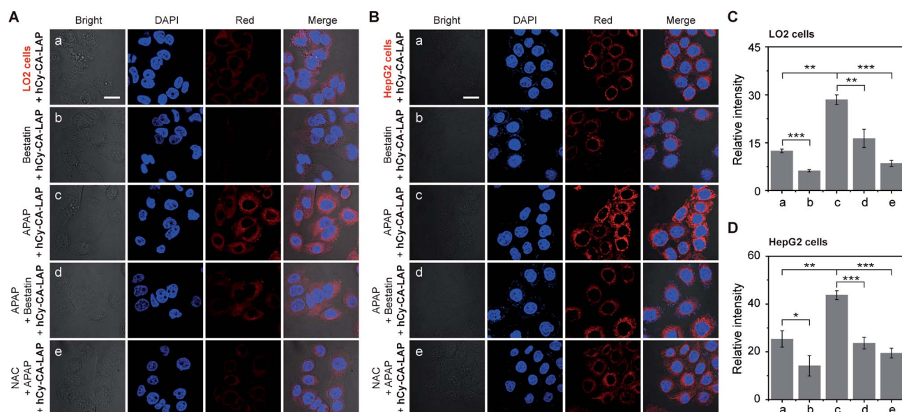
Fig. 3 Fluorescence imaging of LO2 cells (A) and HepG2 cells (B) incubated with hCy-CA-LAP (10 \mu\text{M} ) for 30 min: (a) untreated cells; (b) cells pretreated with 100 \mu\text{M} bestatin for 1 h; (c) cells pretreated with 1 mM APAP for 12 h; (d) cells pretreated with 1 mM APAP for 12 h, and then treated with 100 \mu\text{M} bestatin for 1 h; (e) cells pretreated with 100 \mu\text{M} NAC for 1 h, and then treated with 1 mM APAP for 12 h. (C) and (D) Relative fluorescence intensity of the corresponding fluorescence images in panels A and B, \lambda_{\text{ex}} = 639 \text{ nm} , \lambda_{\text{em}} = 663\text{--}738 \text{ nm} . Scale bar: 25 \mu\text{m} . * P < 0.05 , ** P < 0.01 , and *** P < 0.001 .
