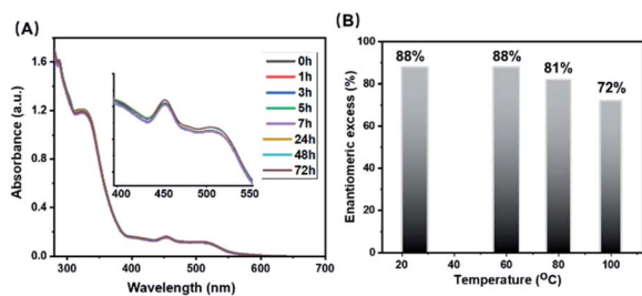
Fig. 6 (A) Thermal stability of rac - 3a at 60 °C in acetonitrile monitored by UV-vis spectroscopy; (B) chiral stability of 3a-en-1 in methanol after treatment at different temperatures for 1 h. The enantiomeric purity after heating was examined by chiral HPLC.
