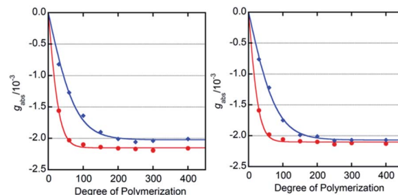
Fig. 3 CD intensities ( g_{\text{abs}} at 367–371 nm at 293 K) of PQX(n) ( \text{ca. } 7 \times 10^{-4} M based on monomer units, n = 30, 60, 100, 150, 200, 250, 300 , and 400) in THF ( \blacklozenge ) and MTBE ( \bullet ) in the presence of TFAc-L-Pro-OMe (left) and Ac-L-Pro-OMe (right) (10 mol%).
