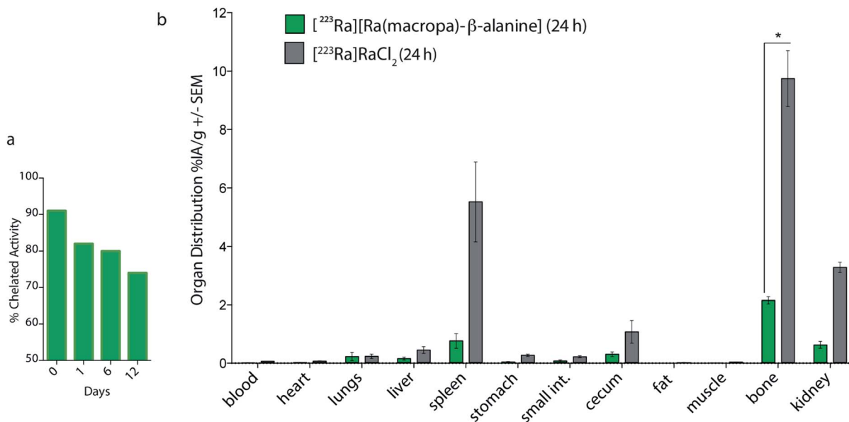
Fig. 6 In vitro and in vivo evaluation of [\text{}^{223}\text{Ra}][\text{Ra}(\text{macropa-}\beta\text{-alanine})] . (a) Stability of [\text{}^{223}\text{Ra}][\text{Ra}(\text{macropa-}\beta\text{-alanine})] over the course of 12 days in human serum at 37 \text{ }^\circ\text{C} . (b) Organ distribution of [\text{}^{223}\text{Ra}][\text{Ra}(\text{macropa-}\beta\text{-alanine})] at 24 h p.i. Significant differences in osseous (* p < 0.005 ), splenic, and renal uptake were observed in comparison to the control [\text{}^{223}\text{Ra}]\text{RaCl}_2 .
