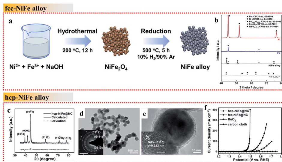
Fig. 3 Examples of NiFe alloys with different crystal phases in the OER. (a) Schematic illustration of the fcc NiFe alloy fabrication process. (b) XRD patterns of Ni, Fe, fcc NiFe alloy and NiFe 2 O 4 . Reproduced from ref. 48 with permission from Elsevier, Copyright 2019. (c) XRD pattern. (d and e) TEM images. The inset of (d) shows the SAED pattern, scale bar is 5 nm -1 . The inset of (e) shows the HRTEM image, scale bar: 2 nm. (f) OER polarization curves recorded on different electrodes. Reproduced from ref. 51 with permission from John Wiley and Sons, Copyright 2019.
