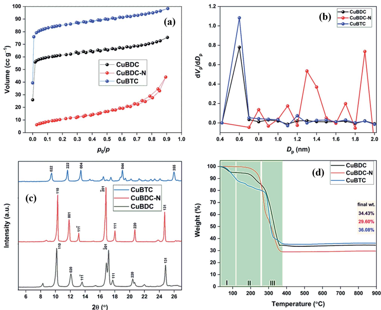
Fig. 3 (a) N_2 adsorption–desorption isotherms at -196^\circ\text{C} ; (b) pore size distribution; (c) XRD patterns; (d) TGA patterns of Cu-MOFs.
