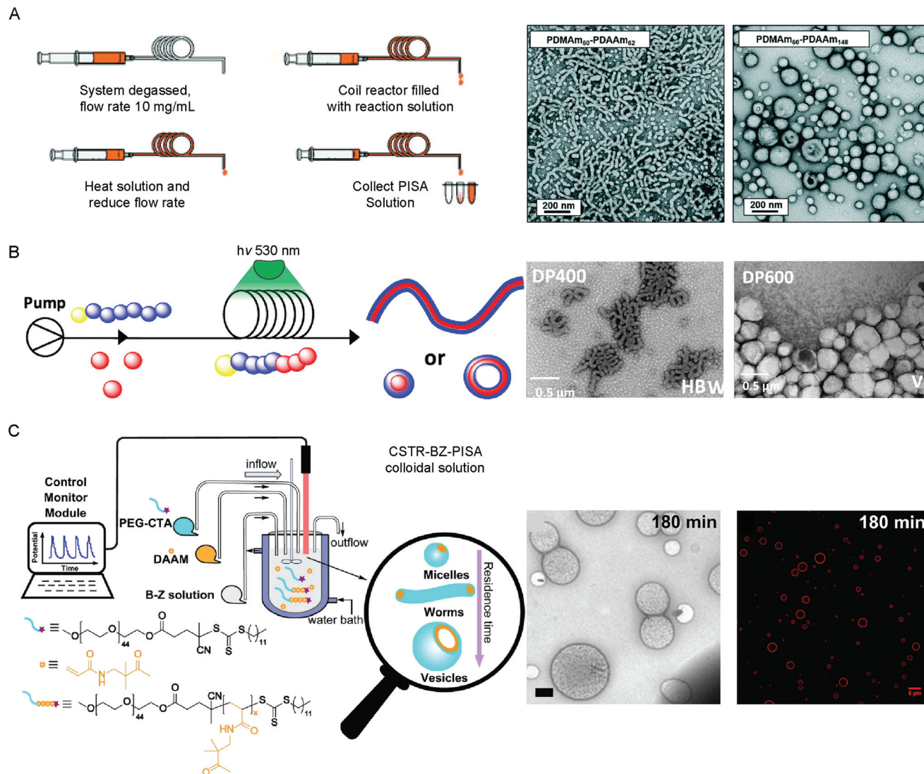
Fig. 4 Methods used to produce vesicles by PISA in flow by (A) thermal-initiated RAFT polymerization of DAAM from \text{PDMAm}_{50} mCTA. Adapted with permission from ref. 84. Copyright 2019 Royal Society of Chemistry. (B) Photo-initiated PET-RAFT of diacetone-stat-dimethyl acrylamide from a PDMA trithiocarbonate mCTA. Reproduced with permission from ref. 86. Copyright 2019 American Chemical Society. (C) BZ-initiated PISA of DAAM from a \text{PEG}_{44} trithiocarbonate mCTA using a CSTR in flow. Scale bar = 500 nm (TEM image) and 5 \mu\text{m} (fluorescence image). Reproduced with permission from ref. 29. Copyright 2019 Springer Nature.
