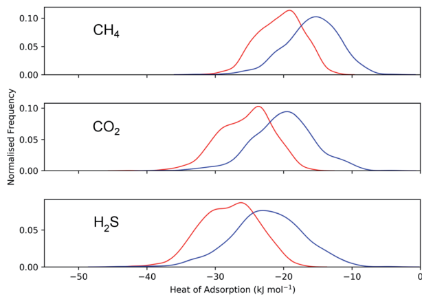
Fig. 8 Distribution of Q_{st}^0 for \text{CH}_4 , \text{CO}_2 and \text{H}_2\text{S} in the MOFs above (red) and below (blue) the 2008 \text{CO}_2/\text{CH}_4 Robeson limit.
